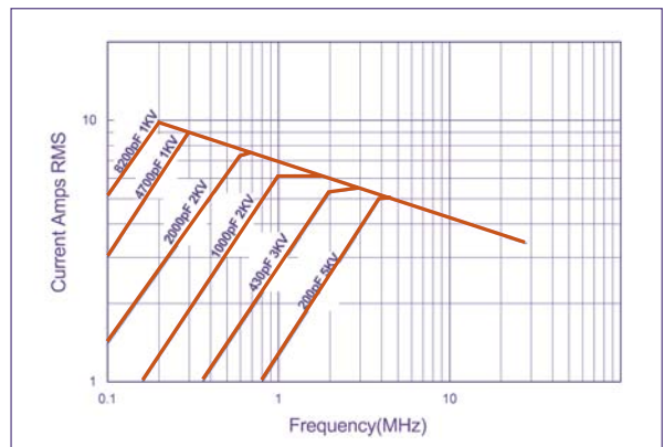
DLC70G Wire Terminals Rated Current vs Frequency
