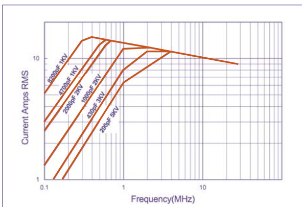
70G Strip Terminals Rated Current vs Frequency
