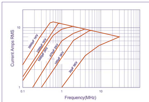
DLC70F Strip Terminals Rated Current vs Frequency
