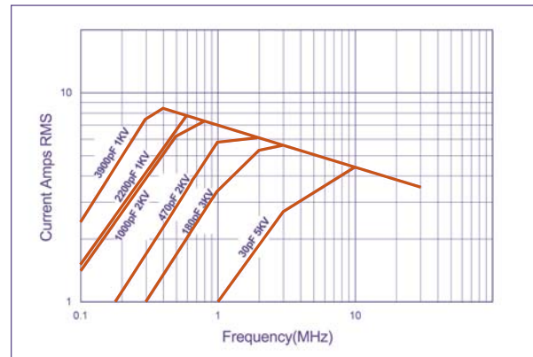
DLC70F Wire Terminals Rated Current vs Frequency
